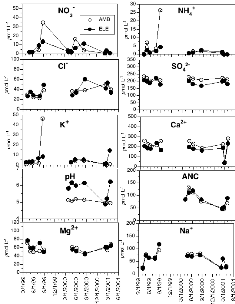
Figure 1. Soil solution concentrations under ambient and elevated \text{CO}_2 . See Table 6 for statistical analyses.
